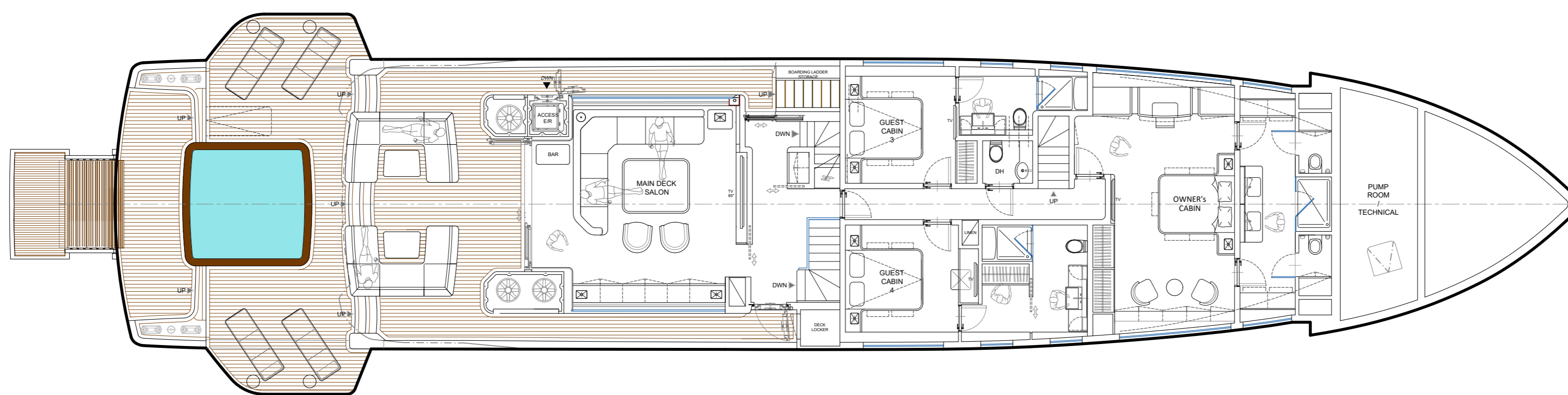
MAIN DECK
