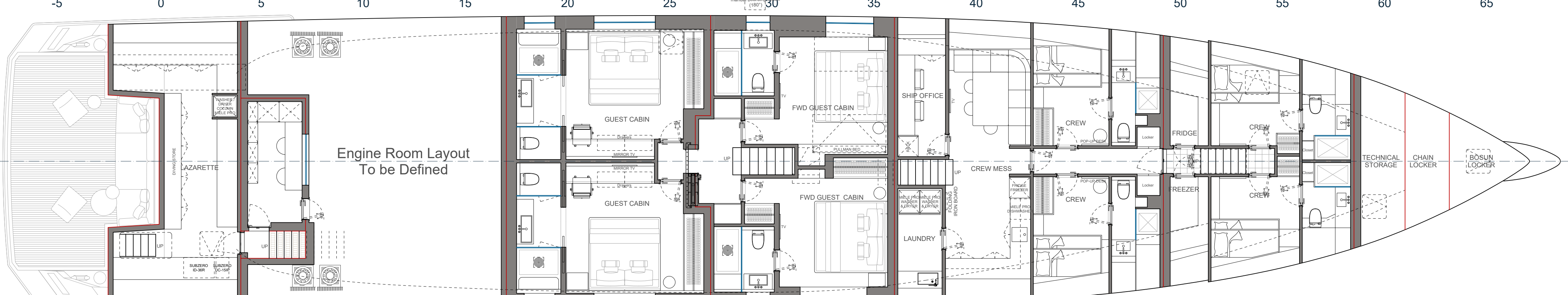
-5 0 5 10 15 20 25 30 35 40 45 50 55 60 65 70 LOWER DECK
