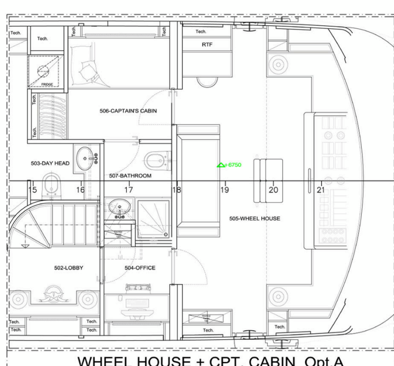
Wheel House - Central sofa/ Capt. Cabin - + Wardrobe
